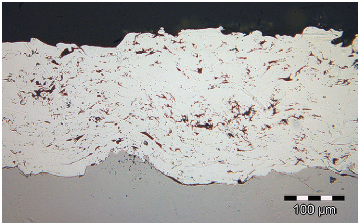
Photomicrograph cross-section of a typical, high quality TSA coating produced using Oerlikon Metco equipment and TSA wire.
